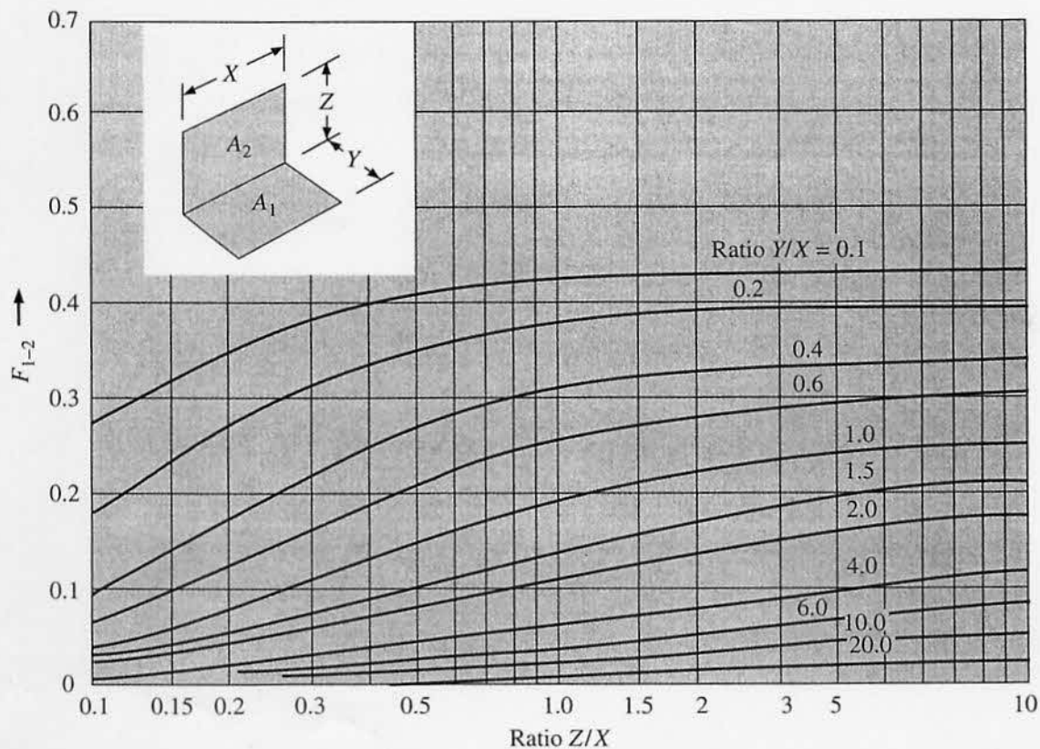
Figure 8-14 | Radiation shape factor for radiation between perpendicular rectangles with a common edge.
