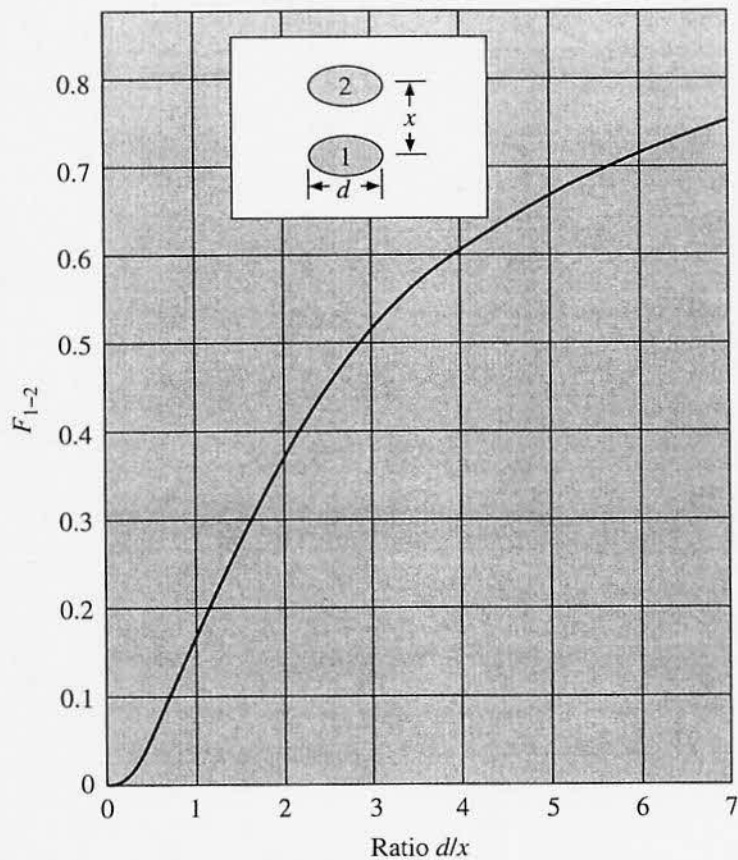
Figure 8-13 | Radiation shape factor for radiation between parallel disks.
